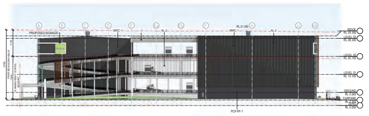
3 SOUTH (CANAL RD) ELEVATION 1:400
