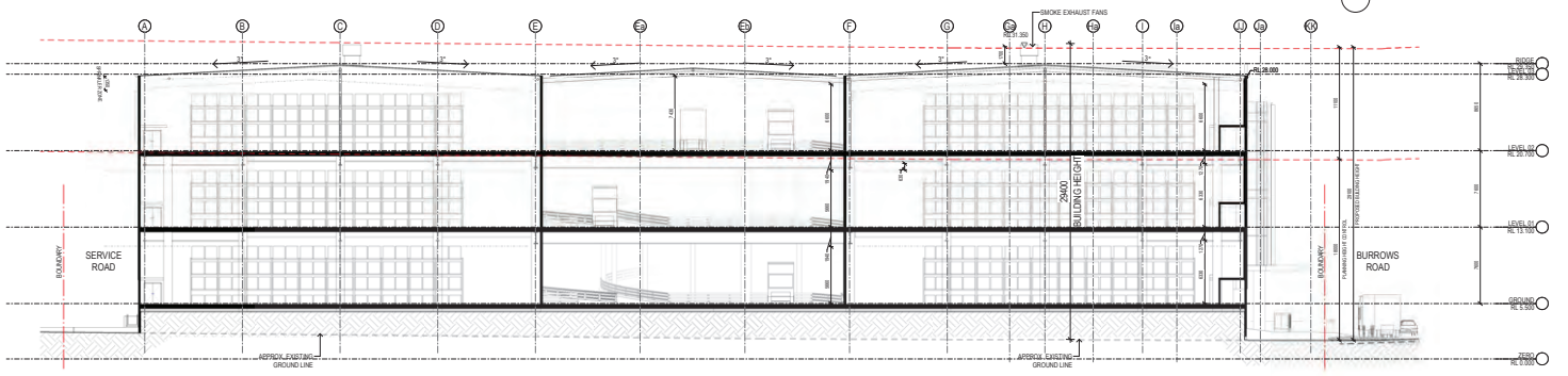
1 SECTION 1 1:200
