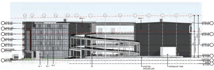
2 NORTH ELEVATION 1:400
